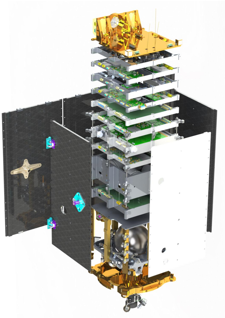
S-75 Platform exploded view
